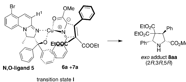
Scheme 2. Proposed transition state leading to the major product exo - 8aa .
